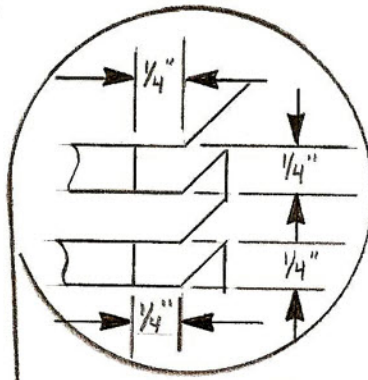
BOX JOINT
