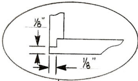
DADO JOINT
